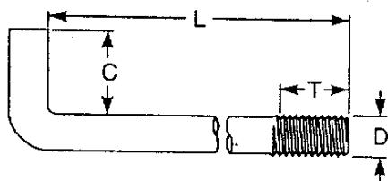
Hook Bolt, Right Angle Bend (DxLxCxT)
