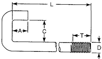
Hook Bolt, Square Bend (DxLxCxAxT)
