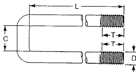
U-Bolt, Square Bend (DxLxCxT)
