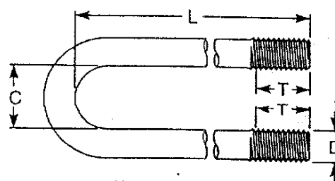
U-Bolt, Round Bend (DxLxCxT)
