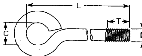
Eye Bolt, Closed (DxLxCxT)
