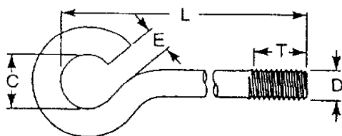
Eye Bolt Open (DxLxCxExT)
