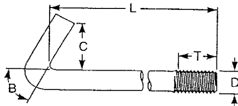
Hook Bolt, Special (DxLxCxTxB) (B expressed in degrees)
