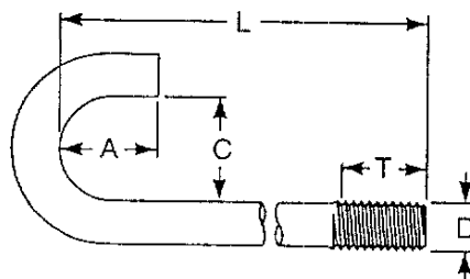
Hook Bolt, Round Bend (DxLxCxAxT)
