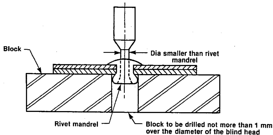
FIG. 4 MANDREL RETENTION TEST FIXTURE
