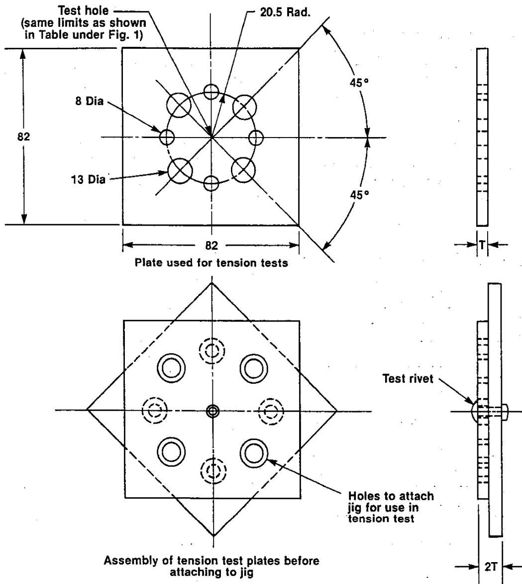
FIG. 2 TEST FIXTURE FOR TENSILE TESTING BLIND RIVETS
