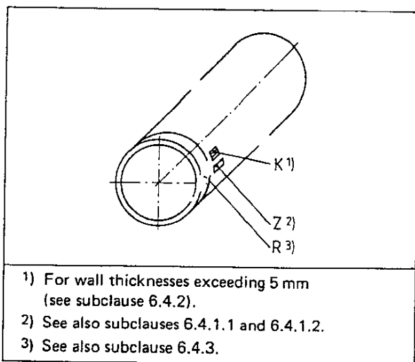
Figure 1. Sampling points and location of test pieces
