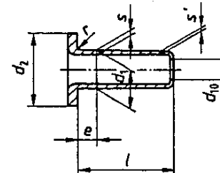
Drawn from strip (C 2)
