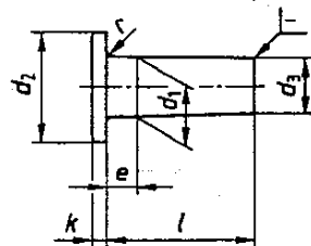
Type A, solid rivet
