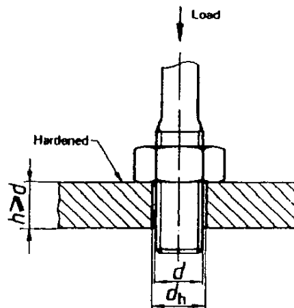
Figure 2 — Axial compressive test
