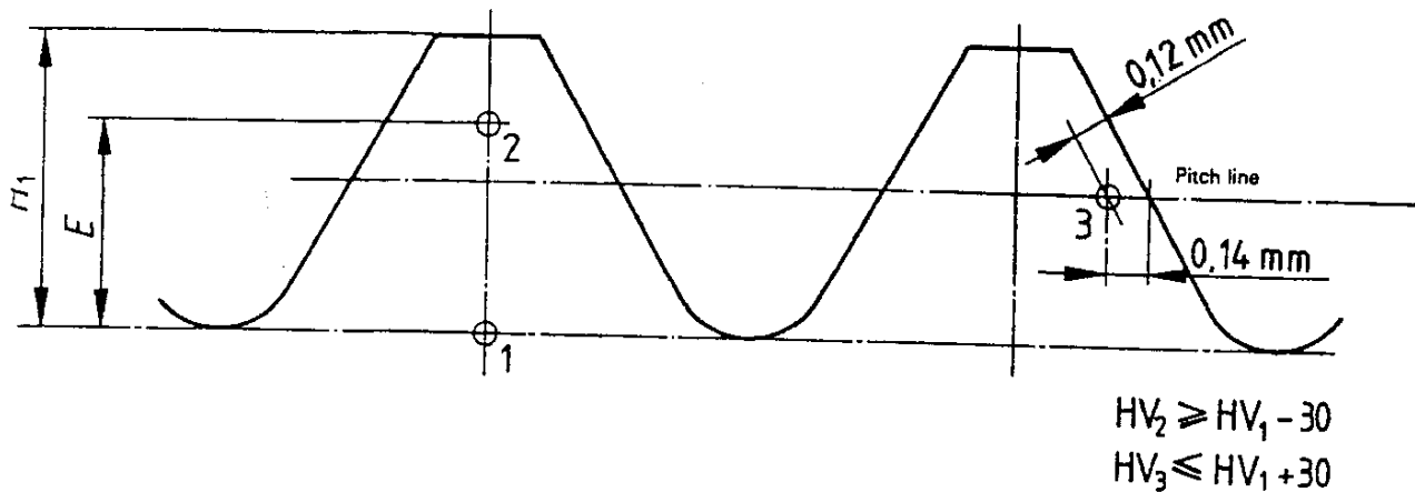
Figure 6 – Hardness measurements for decarburization test
