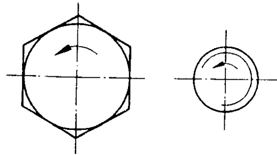
Figure 10 – Left-hand thread marking
